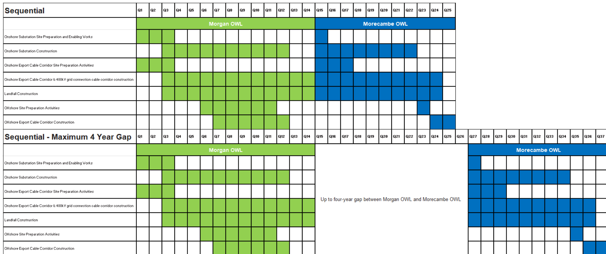
Plate 3.3: Sequential Construction Scenario indicative construction programme for the Morgan Offshore Wind Project: Transmission Assets and Morecambe Offshore Windfarm, including gap of up to four years
